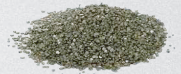
Energetic compound
